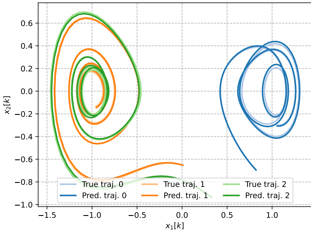
Random Fourier features: true and predicted trajectories
