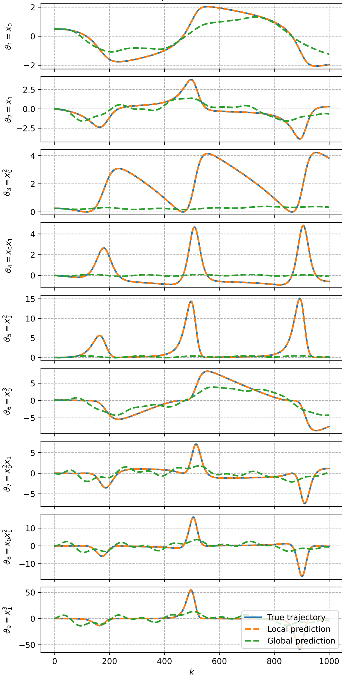
True and predicted lifted states
